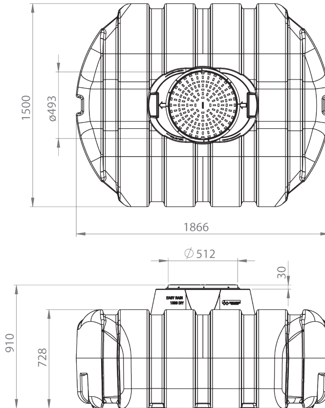
Easy-Rain 1500L tank dimensions.
