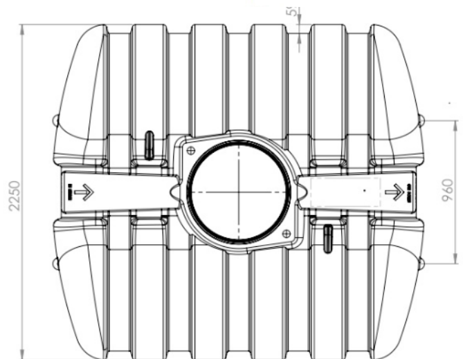
5000L tank dimensions.
