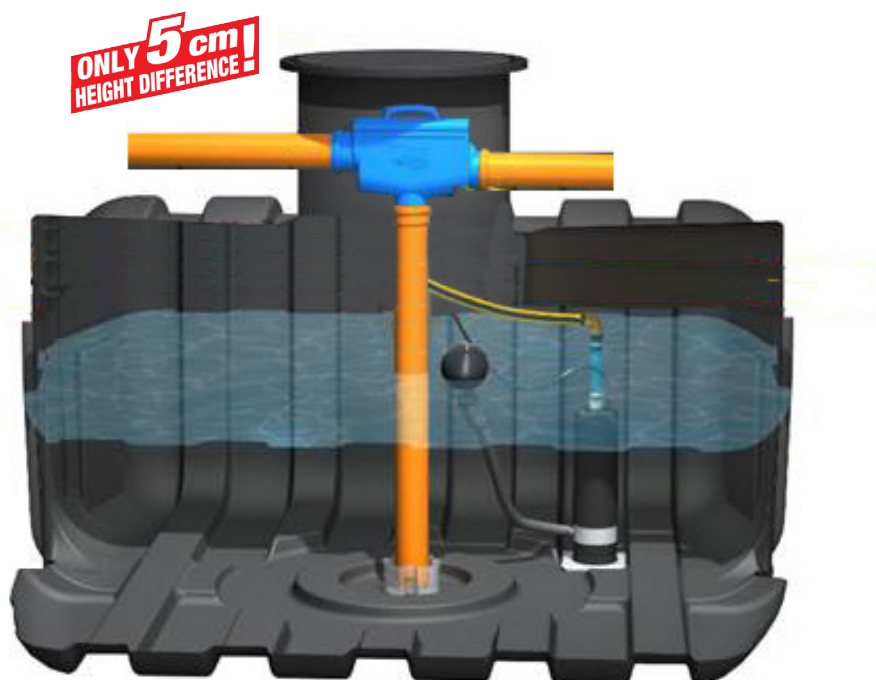
The LineAr filter unit can be fitted either in the turret or inside the tank itself
