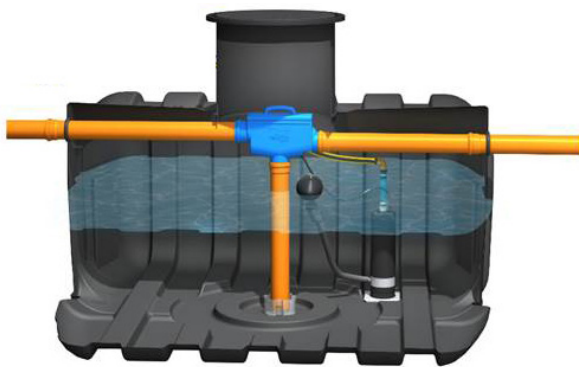
5000 litre flat tank with internal filter unit
