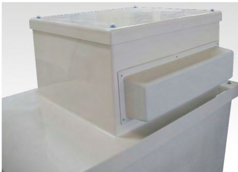
Raised valve housing with screened weir overflow giving a type AB air gap, can be fitted with drop-arm equilibrium float valve or Keraflo valve where required.
