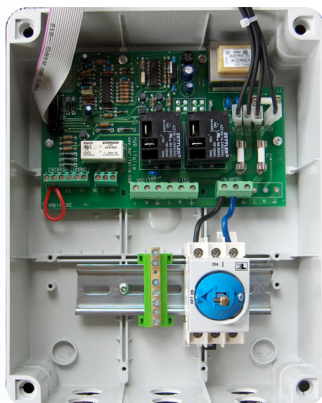
Panel internals with terminal block and DIN rail
