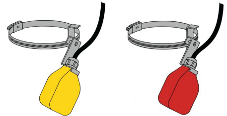
Precision float switches c/w clamps for attaching to pumps. Red body provides dry-run protection, yellow body controls mains water top-up.
